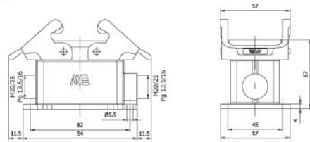
29055 29055S DUVAR GÖVDE (Çift Giriş) Housing (Surface Mounting - Two Entries)
