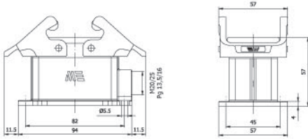
29054 29054S DUVAR GÖVDE Housing (Surface Mounting)
