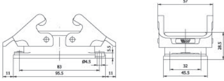
29054 29054S DUVAR GÖVDE Housing (Surface Mounting)
