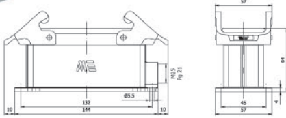
29059 29059S DUVAR GÖVDE (Çift Giriş) Housing (Surface Mounting - Two Entries)
