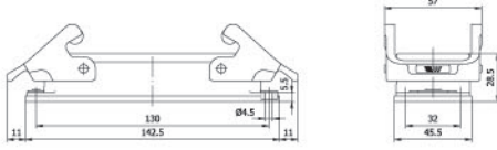
29058 29058S DUVAR GÖVDE Housing (Surface Mounting)
