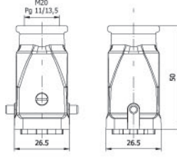
UZATMA PRİZİ Hood With Female Insert
