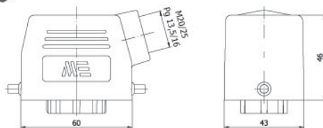
403092 UZATMA PRİZİ-2 (Yandan Girişli) Hood With Female Insert (Side Entry)
