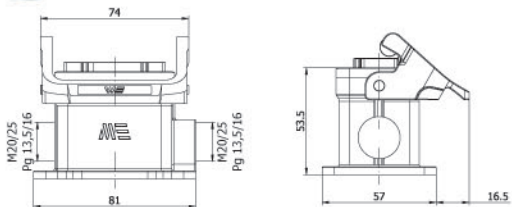
403099 DUVAR FİŞİ (Çift Giriş) Housing With Male Insert (Surface Mounting Two Entries)
